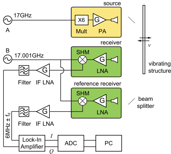
Figure 1 : Flowchart of the mm-wave Doppler heterodyne radar sensor.
