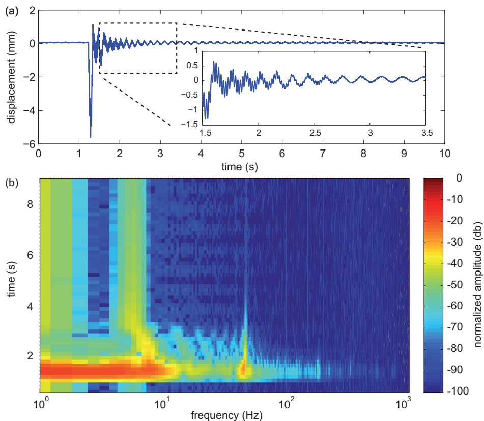
Figure 5 : (a) Displacement of the nonlinear motion experiment (b) Short-Time-Fourier-Transform of the displacement signal.
