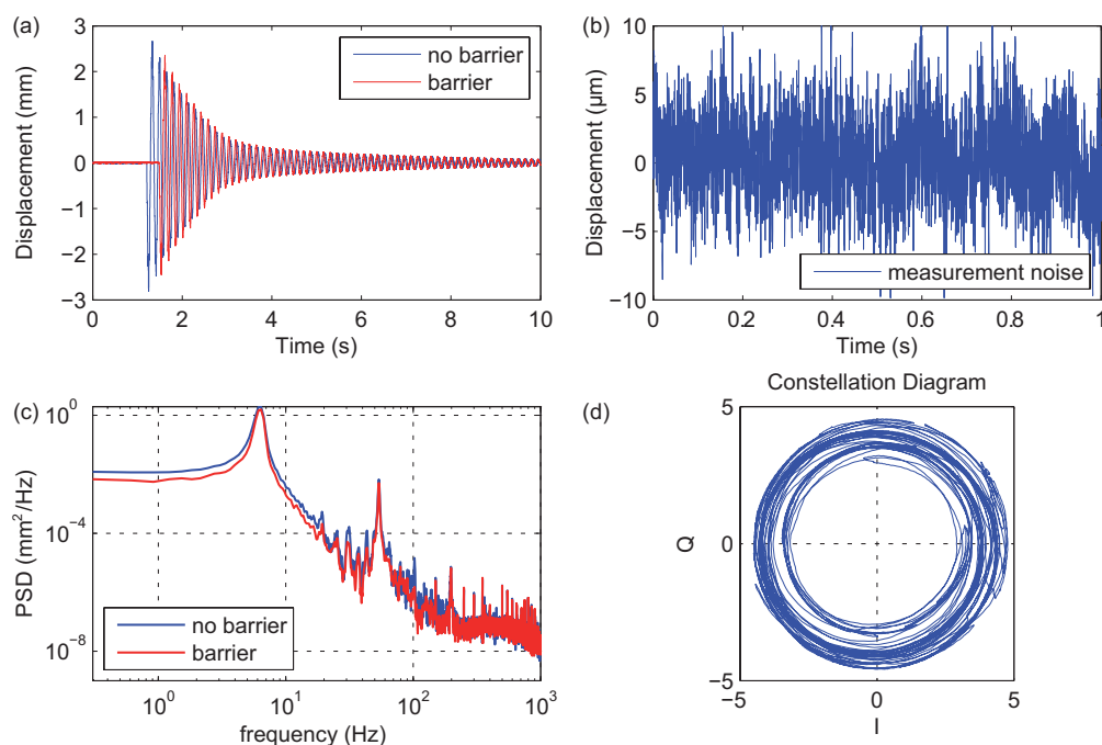
Figure 3 : (a) Displacement for barrier / no barrier (unfiltered); (b) close-up of the displacement to show the measurement noise; (c) Comparison of power spectral densities; (d) centred constellation diagram.
