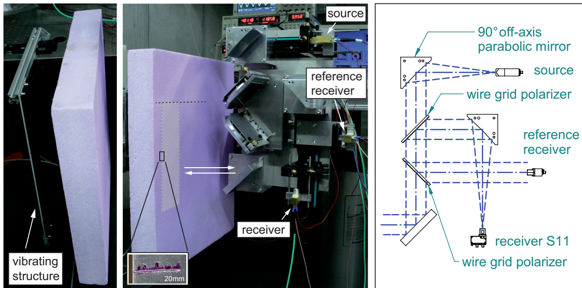
Figure 2 : (left) Experimental setup for mm-wave remote sensing; submillimeter-vibrations are found behind a barrier of 80mm thick polystyrene foam; (right) Millimeter-wave path within the experimental setup.
