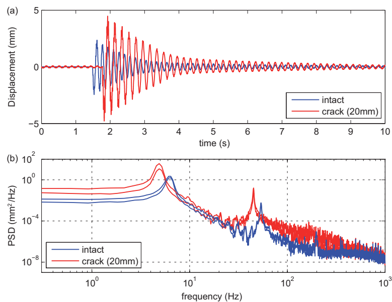
Figure 4 : (a) Displacement measurements (b) Power spectral densities for the intact and the damaged structure (two measurements for each case).
