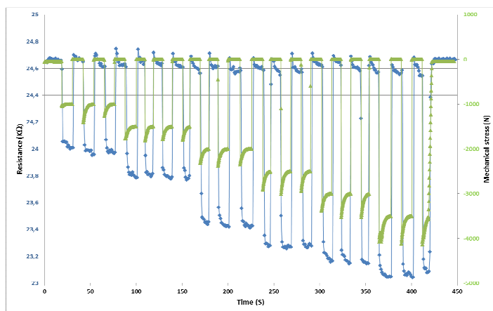
Figure 4: Piezoresistive response of C/sep-MWCNTs-asphalt composite
