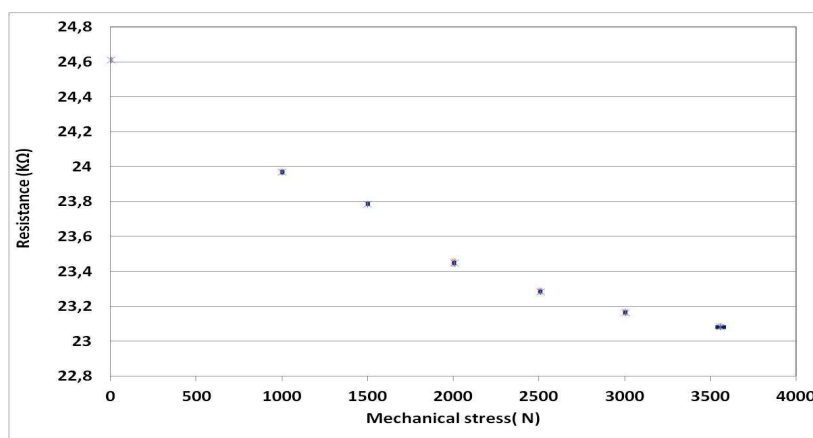
Figure 5: Piezoresistive behaviour of C/sep-MWCNTs-asphalt composite
