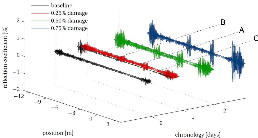
Figure 4. Baseline residual signals corresponding to raw signals of Figure 3.
