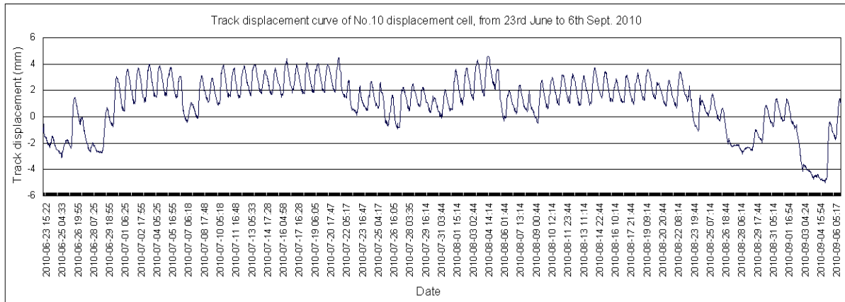
Fig.11 Curve of track displacement measured by the displacement cell No.10 in 75 days
