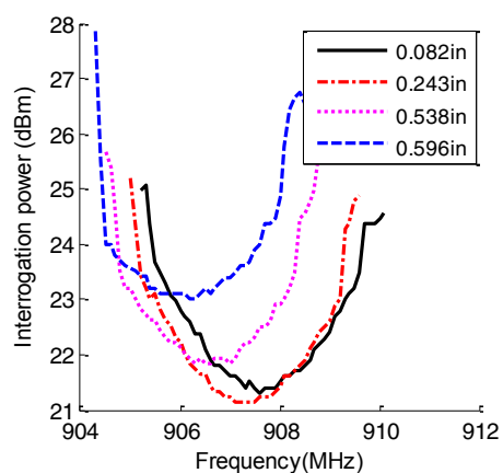
(a) Average interrogation power and threshold (b) Resonance frequency change with crack length
