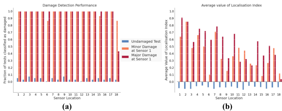
Figure 4: (a) Damage detection using low-cost machine learning based method, (b) damage localization using the OCSVM localization index.
