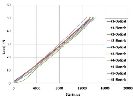
Figure 10: Comparison of load-strain curves measured by optical fibre sensor and electrical-resistance sensor
