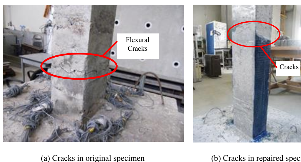
Figure 4: Cracks in plastic hinge zone of original pier model and at top of CFS of repaired pier model
