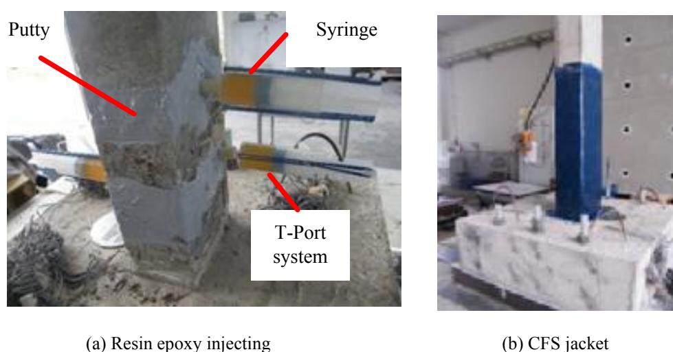
Figure 3: Repairing method of damaged pier by resin epoxy injection and CFS jacketing
