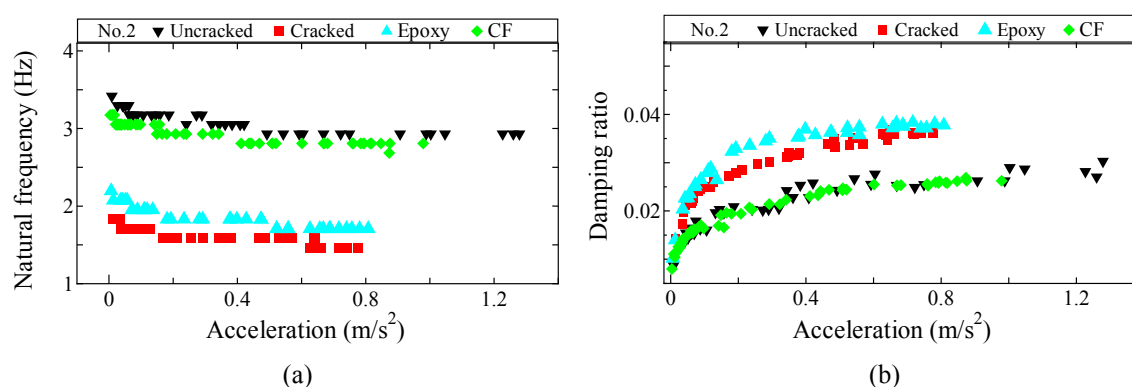
Figure 8: Maximum acceleration response vs natural frequency and damping ratio
