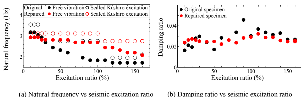
(a) Natural frequency vs seismic excitation ratio (b) Damping ratio vs seismic excitation ratio
