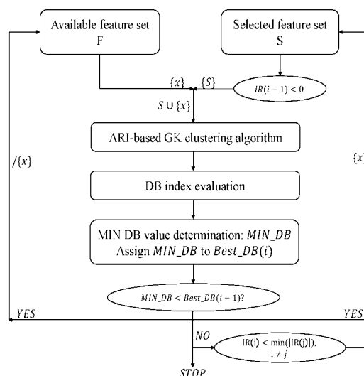
Figure 2: Progressive feature selection diagram
