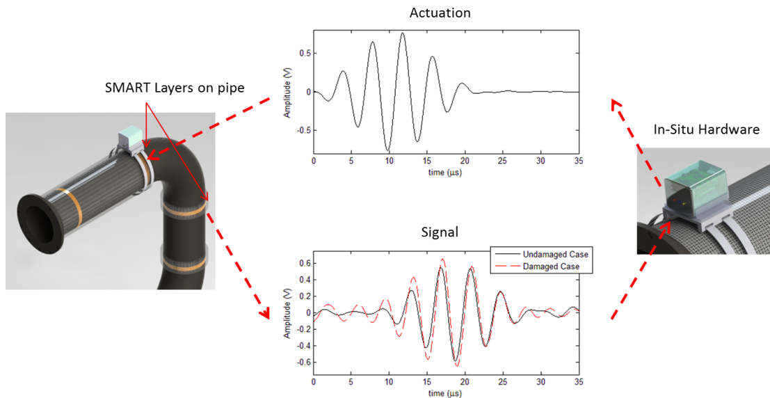
Figure 2: Principle of RAPID system
