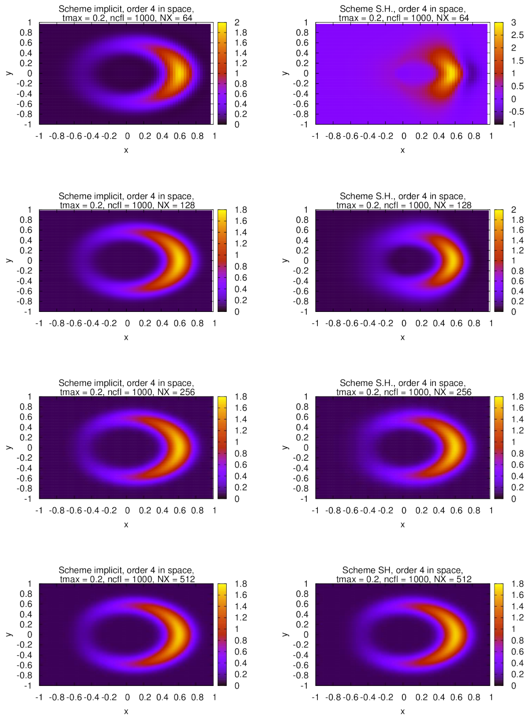
Figure 13: Diffusion on a ring at t_{\max} = 0.2 , for implicit and SH time schemes, with N_x = 64, 128, 256 and n_{\text{CFL}} = 1000 fixed.
