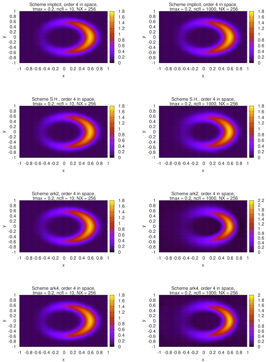
Figure 11: Diffusion on a ring at t_{\max} = 0.2 , for semi implicit and implicit time schemes, with N_x = 256 and n_{\text{cfl}} = 10 and 1000.
