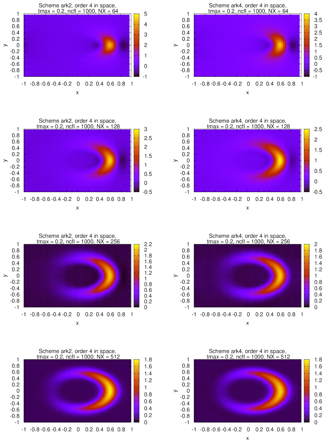
Figure 14: Diffusion on a ring at t_{\max} = 0.2 , for ARK2 and ARK4 time schemes, with N_x = 64, 128, 256 and ncfl = 1000 fixed.
