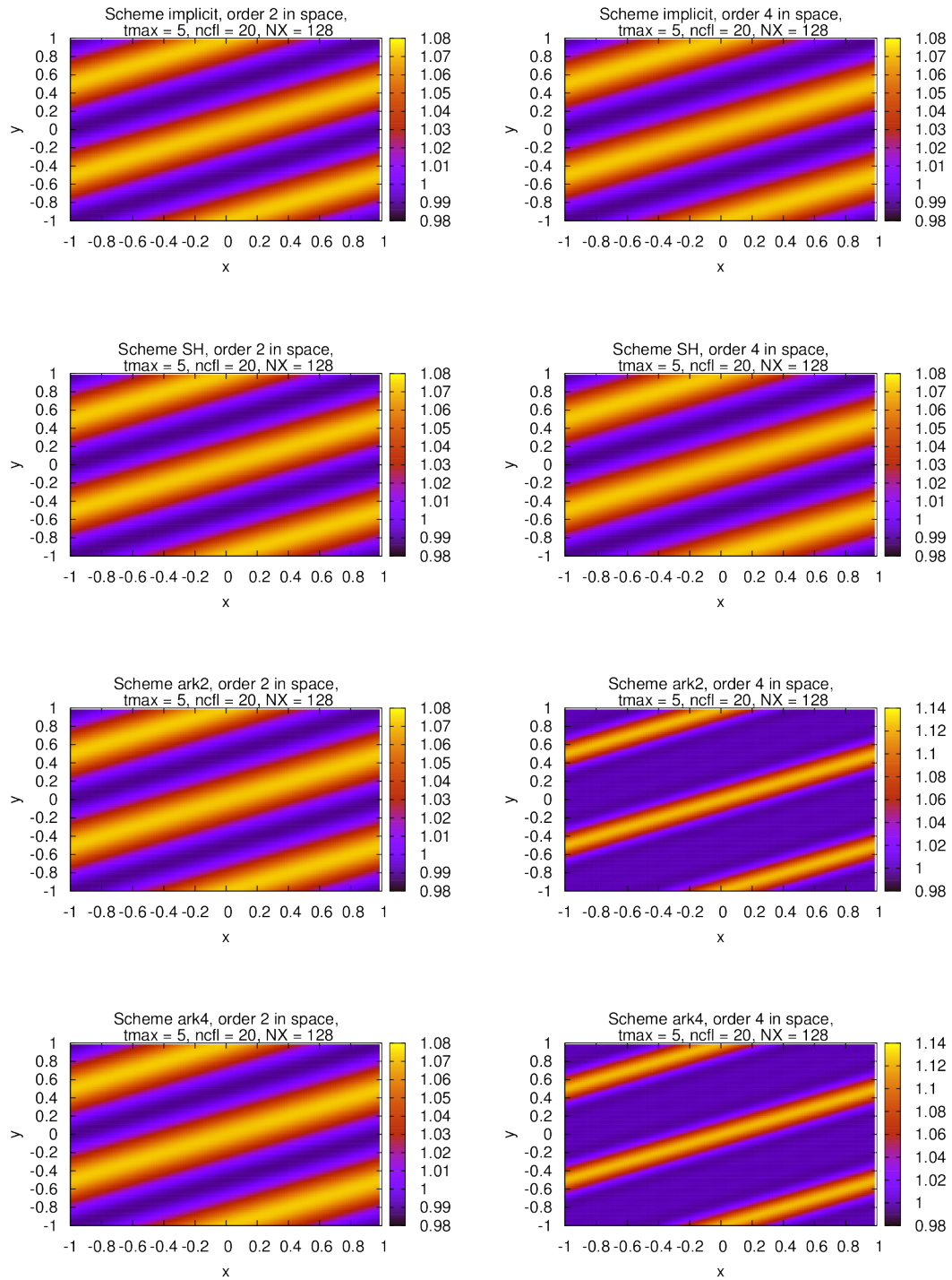
Figure 17: Diffusion on a periodic band at t_{\max} = 5 , for different time scheme, with N_x = 128 and ncl = 20 .
