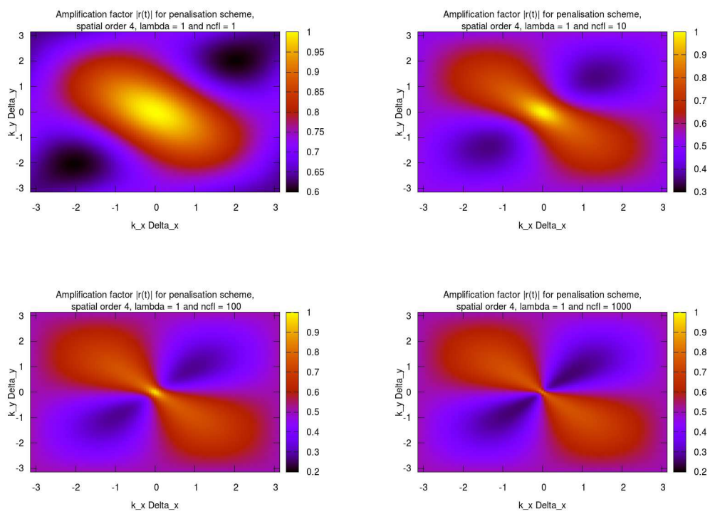
Figure 5: Amplification factor |r(t)| for n\text{ CFL} = 1, 10, 100, 1000 for ARK scheme of order 4 in space.
