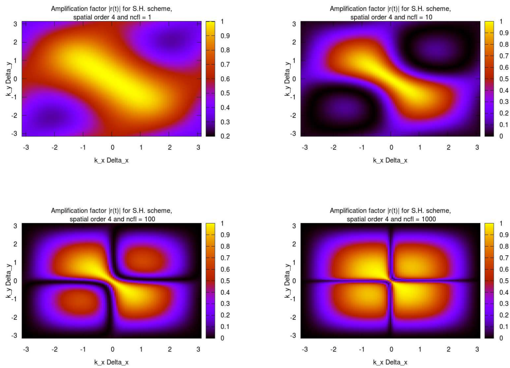
Figure 3: Amplification factor |r(t)| for ncf=1, 10, 100, 1000 for SH scheme of order 4.
