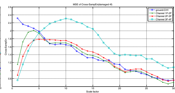
Figure 11 Cross-SampEn trend analyzed from signal of different floors of damaged 4F case
