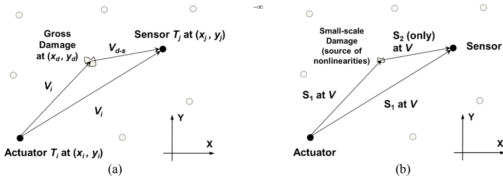
Figure 1: (a) Part of a transducer network with gross damage: the idea of using TOF for damage localization; and (b) using TOF of nonlinear Lamb waves for small-scale damage localization
