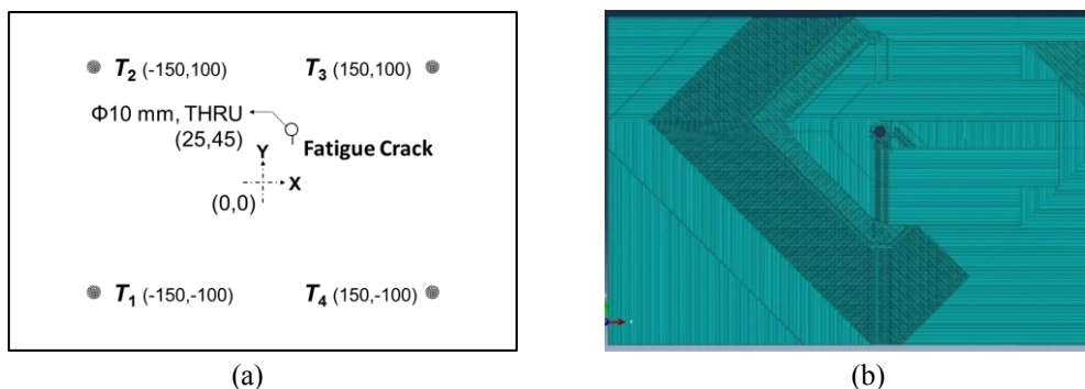
Figure 2: (a) Schematic of the simulated aluminum plate with a rivet hole and four transducers (in mm, crack length exaggerated); and (b) meshed FE model of the plate.
