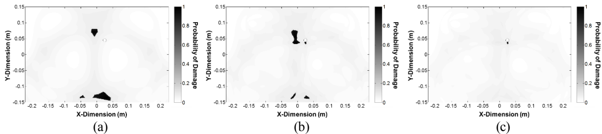
Figure 7: Diagnostic images using DI_S with (a) w_{NL} = 0 ; (b) w_{NL} = 0.4 ; and (c) w_{NL} = 0.5 ( \kappa = 0.9 for all)
