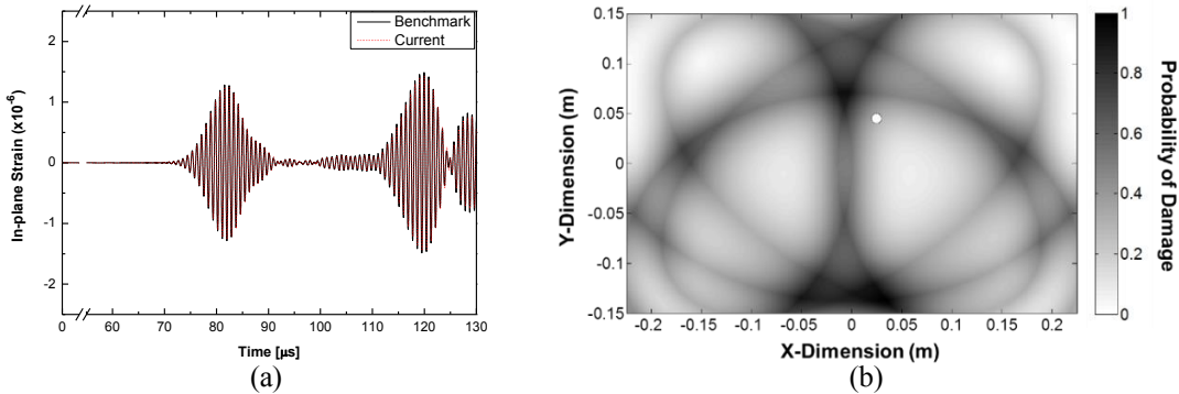
Figure 3: (a) Time series via T_1 - T_4 ; and (b) Imaging using TOFs of linear signals from simulation.
