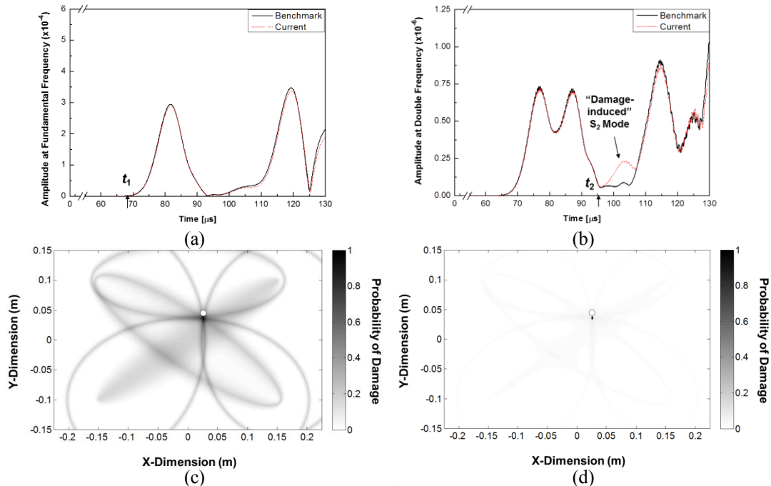
Figure 4: Amplitude profiles of signals via T_1 - T_4 at (a) fundamental frequency, and (b) double frequency; (c) a raw diagnostic image using TOFs of second harmonic features; and (d) improved imaging with \kappa = 0.9
