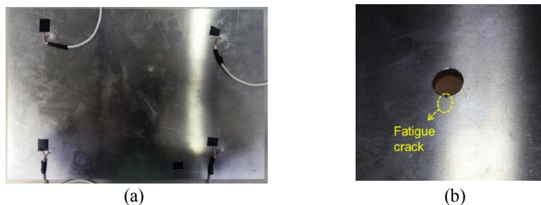
Figure 5: (a) Aluminum plate with a rivet hole; and (b) barely visible crack after fatigue testing
