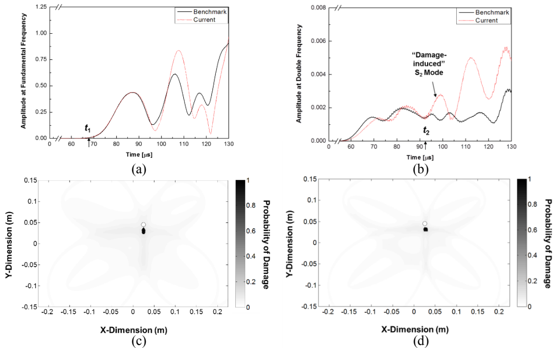
Figure 6: Amplitude profiles of experimental signals via T_1 - T_4 at (a) fundamental frequency, and (b) double frequency; and diagnostic images using TOFs of (c) linear signals, and (d) nonlinear signals, both with \kappa = 0.9
