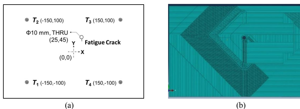
Figure 2: (a) Schematic of the simulated aluminum plate with a rivet hole and four transducers (in mm, crack length exaggerated); and (b) meshed FE model of the plate.
