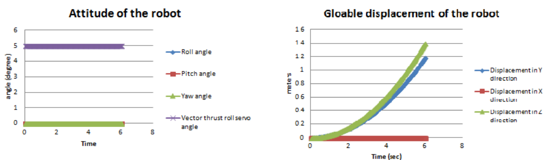
Figure 6: Left: Numerical simulation results of MAV (robot) attitude when vector thrust roll servo is active at 5 degree. (Note: no autopilot control). Right: global displacement of the robot. Note: no undesired x displacement due to no yaw angle created.
