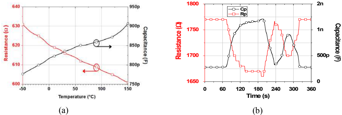
Figure 9: R_p and C_p sensitivity to temperature (a) and deformations (b)
