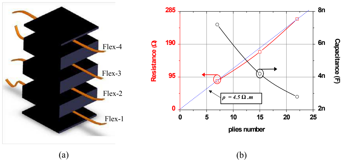
Figure 5: Inter-ply conduction test sample (a), resistance versus plies number (b)
