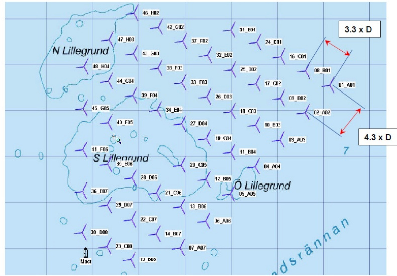
Figure 1 : Lillgrund wind farm and the distribution of the wind turbines [12].
