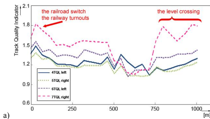
Figure 5: Track condition chart along 1 km near Sochaczew on January 25 th , 2012 in the case of B-bogie – comparing the values of track quality indicator obtained on the right and the left rails
