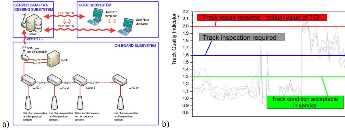
Figure 1: Scheme of Rail Vehicle's and Rail Track Monitoring System (a) and the boundaries track quality indicator values (b)
