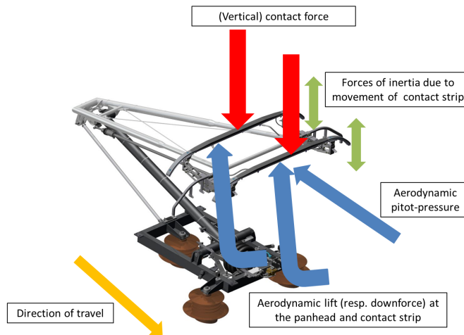
Figure 1 : a) Pantograph and contact force; b) Placement of force sensors on pantograph
