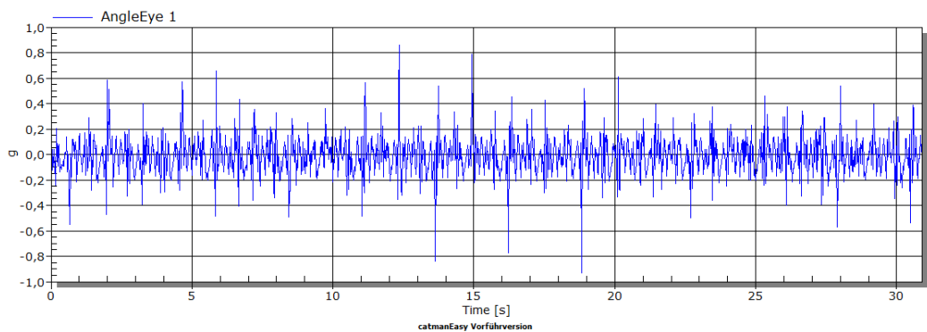
Figure 9 : Measured Acceleration on one contact strip; zig-zag actuation, amplitude 800mm
