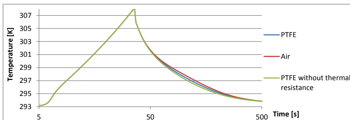
Figure 5: Graph of the temperature in function of the time for defect of different nature and properties.
