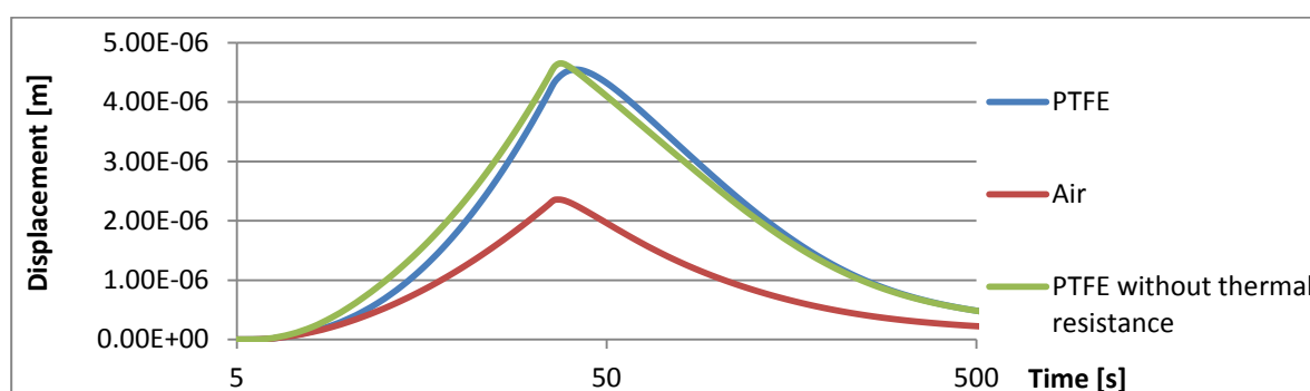
Figure 6: Graph of the out-of-plane displacement in function of the time for defect of different nature and properties.
