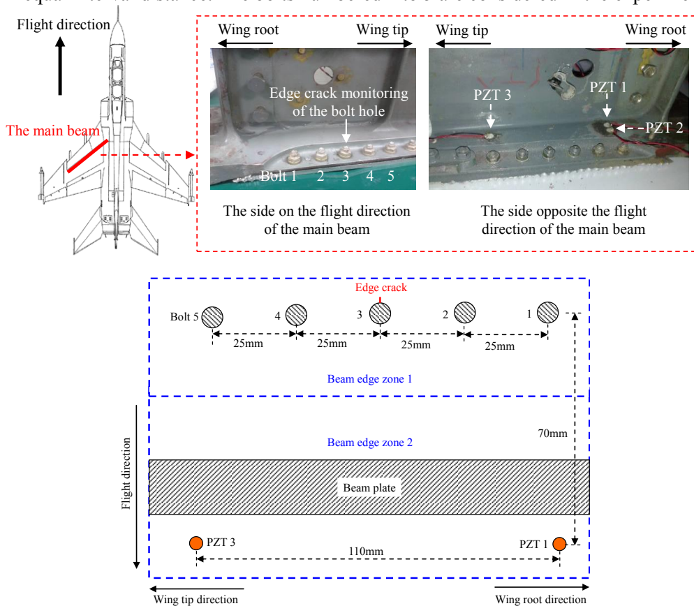
Figure 2: The aircraft main beam and PZTs placement
