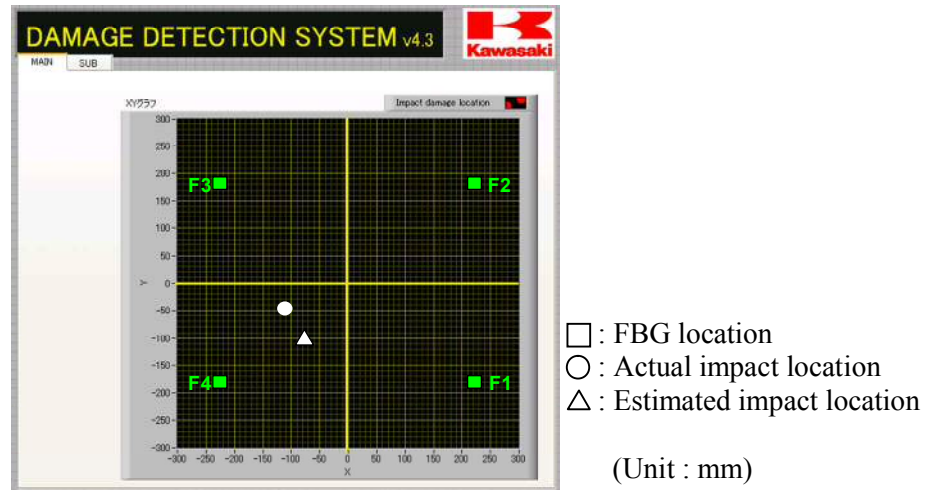
Figure 5: Localization result of impact location under random vibration
