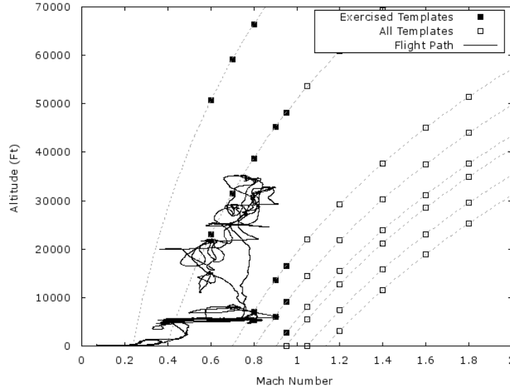
Figure 3 – Locations of the templates on the dynamic pressure bands with an example trajectory shown in black through the flight. envelope. The used templates are shown in solid black squares and unused templates are shown as outline squares.
