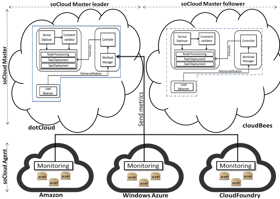
Fig. 4 Conceptual view of a soCloud deployment.
