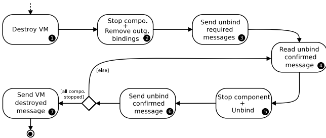
Figure 6: VM Manager Activity Diagram: Down Phase (Destruction)
