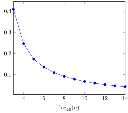
Fig. 4: Average number of generated points divided by n^{\frac{1}{3}} \log^2 n
