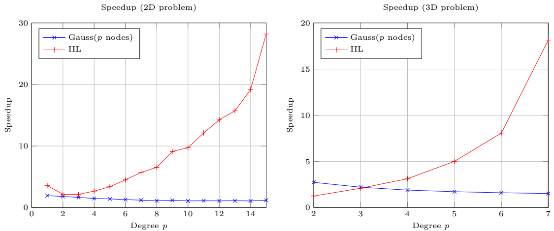
Fig. 13. The experimentally observed speedup for various polynomial degrees: 2D model problem (left) and 3D model problem (right).
