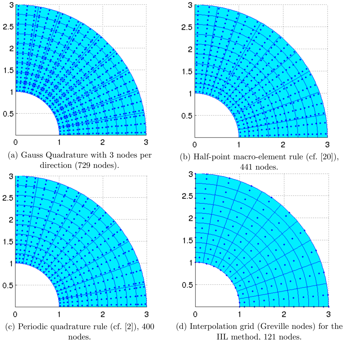
Fig. 2. Evaluation points for different numerical integration rules, for a 9 \times 9 quadratic B-spline discretization of a quarter annulus.
