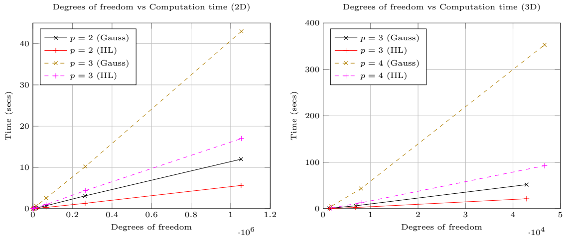
Fig. 10. Linear scaling with respect to the degrees of freedom.
