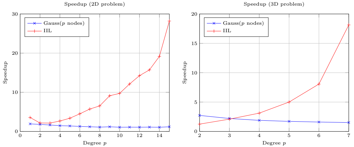
Fig. 13. The experimentally observed speedup for various polynomial degrees: 2D model problem (left) and 3D model problem (right).
