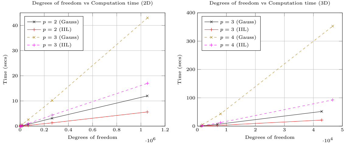
Fig. 10. Linear scaling with respect to the degrees of freedom.
