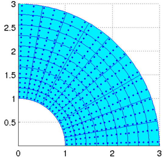
(b) Half-point macro-element rule (cf. [20]), 441 nodes.
