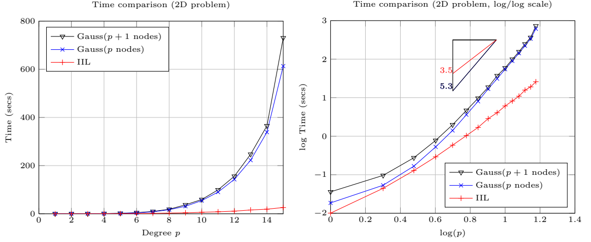
Fig. 11. 2D model problem: Computation time for assembling the stiffness matrices for degree p = 1, \dots, 15 . Standard (left) and doubly logarithmic plot (right)
