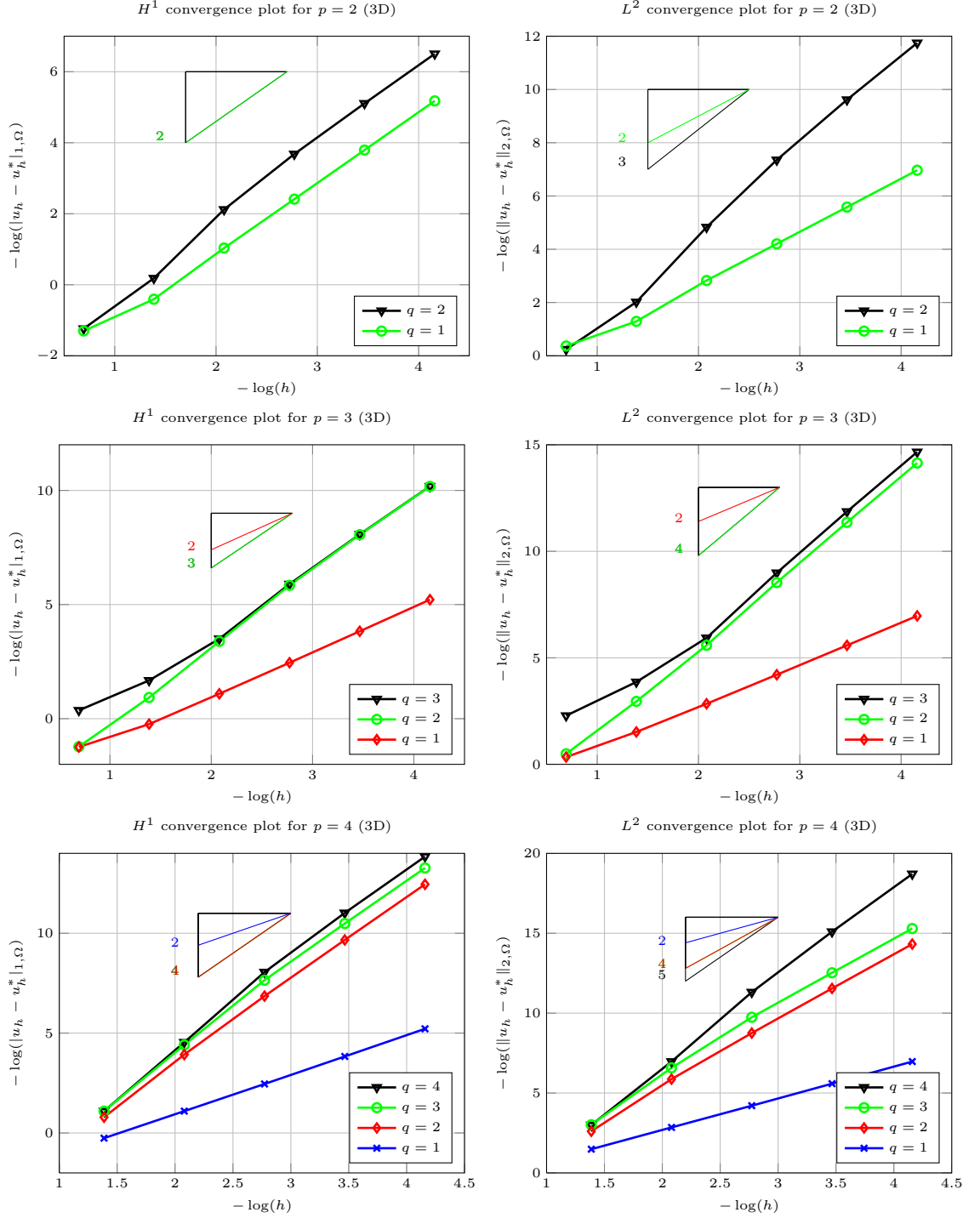
Fig. 8. 3D model problem: Error plots and convergence rates of the IIL method using different degree p = 2, \dots, 4 and q = 1, \dots, p .
