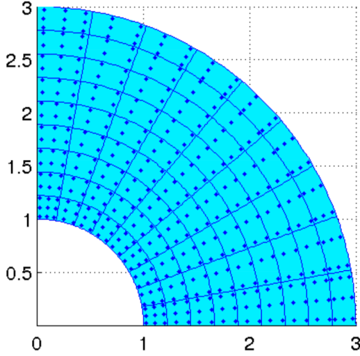
(c) Periodic quadrature rule (cf. [2]), 400 nodes.
