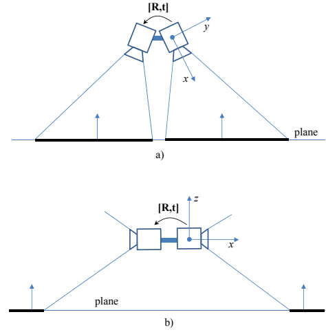
Fig. 3. Different sensor configurations with a pair of cameras: a) Adjacent cameras, b) Opposite cameras.
