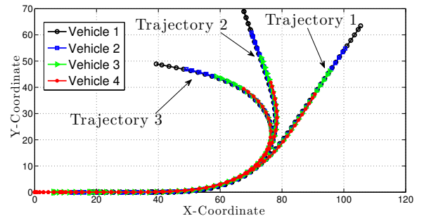
Fig. 8. Four vehicles platoon model in SIMULNK for three different trajectories. Trajectory 1,2 and 3 illustrate the success scenario when the FOV enhancement method is applied, where \theta_F and \theta_R never exceeding \theta_c .
