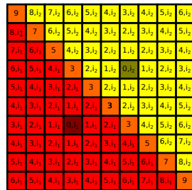
(b) asynchronous computed bisector
