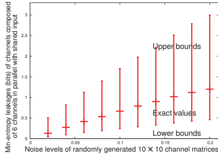
Fig. 4. Min-entropy leakages and their bounds for known channels
