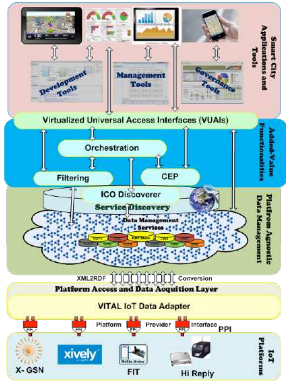
Figure 4: VITAL Platform.
