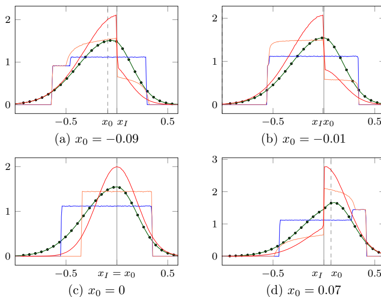
Figure 9: After one time step for different starting points. Density q(t, x_0, \cdot) (black dots) and empirical densities \bar{q}_N(t, x_0, \cdot) in an infinite bimaterial medium with D^- = 5 , D^+ = 2 ( \rho = 2.5 ) and an interface at x_I = 0 . We use different starting points x_0 close to x_I . The time step is \delta t = 0.01 . We used N = 10^7 particles. The colors of the lines follows the convention of Table 5. This graphs shows how the shape of the empirical densities may vary greatly with a starting point close to the interface.
