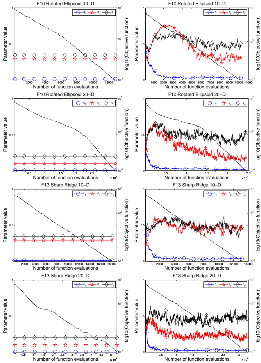
Fig. 2. Evolution of c_1 , c_\mu , c_c (left y-axis) and \log_{10}(\text{objective function}) (right y-axis) of CMA-ES (left column) and self-CMA-ES (right column) on 10- and 20-dimensional Rotated Ellipsoid and Sharp Ridge functions [4]. The medians of 15 runs are shown.
