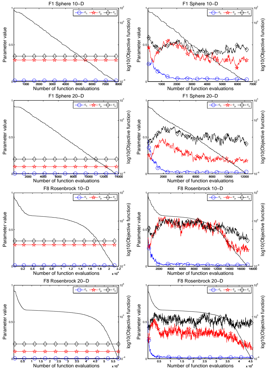
Fig. 1. Evolution of c_1 , c_\mu , c_c (left y-axis) and \log_{10} (objective function) (right y-axis) of CMA-ES (left column) and self-CMA-ES (right column) on 10- and 20-dimensional Sphere and Rosenbrock functions from [4]. The medians of 15 runs are shown.
