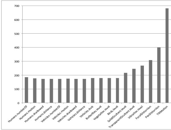
Figure 6: Required time when VANE optimizes one quality attribute.
