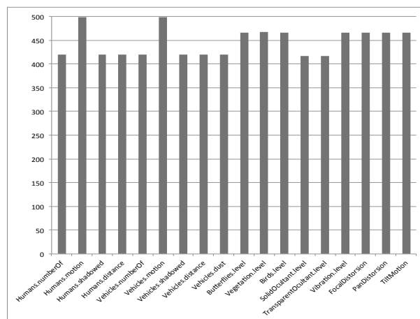
Figure 7: Required number of different configurations when VANE optimizes one quality attribute.
