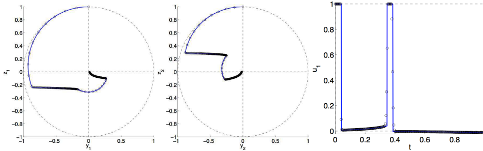
FIG. 12. Blood case with N = 2 spins , \lambda = 1.1 , \varepsilon_{\max} = 0.3 . Solution from direct (dots) and indirect (line) methods. Control structure is 2BS . The rough solution from the direct method is actually quite close to the refined solution from the indirect method.
