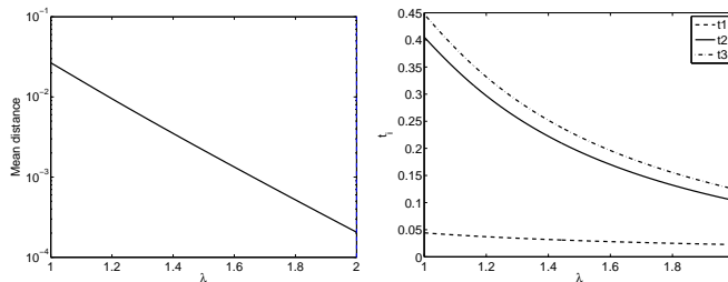
FIG. 13. Homotopy on transfer time (parameter \lambda ) . The mean distance to the origin (left) decreases linearly in log scale. The switching times (right) indicate a decreasing duration t_2 - t_1 for the first singular arc.
