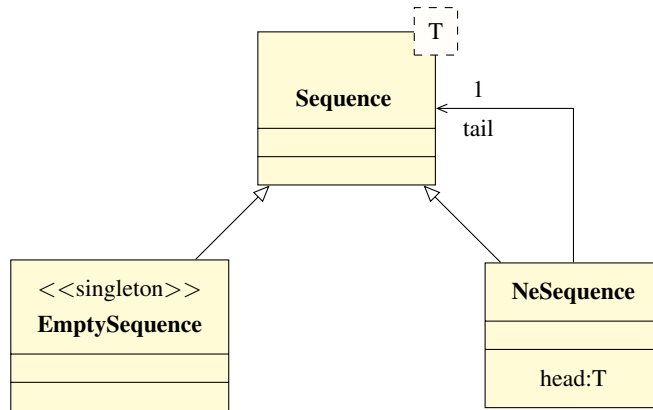
Fig. 4. A diagram for Sequence(T)
