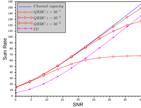
Fig. 3. Sum Rate averaged over 100 MIMO 2 \times 2 Channel realization for UU and QR-PMSVD decomposition. The Channel length was L = 7 , the truncation parameter \mu = 10^{-6} for various \epsilon .
