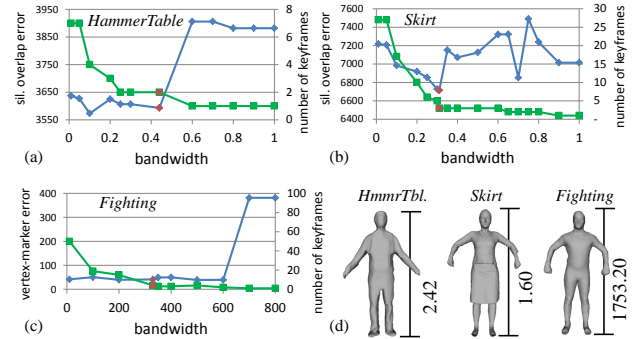
Figure 7. (a-c): performance and the number of keyframes v.s. bandwidth. (d): the heights of the subjects in 3 sequences. Blue curves are the corresponding error (left y -axis) while green curves represent the number of keyframes (right y -axis). (a): HammerTable . (b): Skirt . (c): Fighting . See text for more details.
