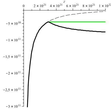
Fig. 13: Actual potential -\Delta V_G(x) (dashed) and apparent asymptotic potential \Delta \tilde{V}_G(x) (plain) for a gravitational walk with realistic setting M_S = 2 \times 10^{42} \text{kg} (1 trillion solar masses), critical z = 3 \times 10^{21} \text{m} (300,000 light-years), in green we display the average value between actual and apparent potential.
