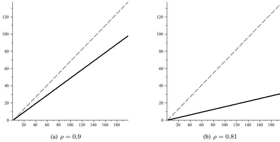
Fig. 4: Actual potential (dashed) and apparent asymptotic potential (plain) for p = 0.2 , two values for \rho greater than 2\sqrt{pq} = 0.8
