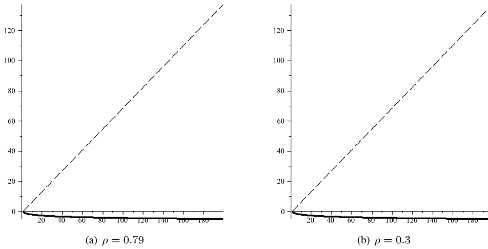
Fig. 5: Actual potential (dashed) and apparent asymptotic potential (plain) for p = 0.2 , two values for \rho smaller than 2\sqrt{pq} = 0.8 .
