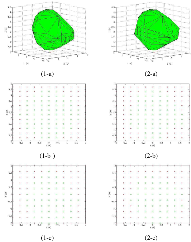
Fig. 10. Experimental evaluation of the convergence domain. Result are given for zero z -axis rotation in column (1) and 30^\circ z -axis rotation in column (2). The first row shows for both cases the convex hull of the points from where the system successfully converged. Rows (b) and (c) shows slices at the desired y and z planes respectively. The poses that converged are shown by green circles and those that diverged by red crosses.
