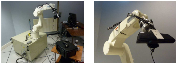
Fig. 3. ADEPT Viper robotic system equipped with a Microsoft Kinect sensor.
