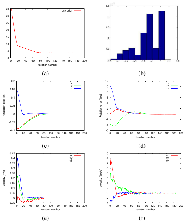
Fig. 7. First experiment. (a) Task error, (b) histogram of depth errors (m) corresponding to the initial frame, (c) translational part of positioning error, (d) rotational part of positioning error, (e) translational velocities, (f) rotational velocities.
