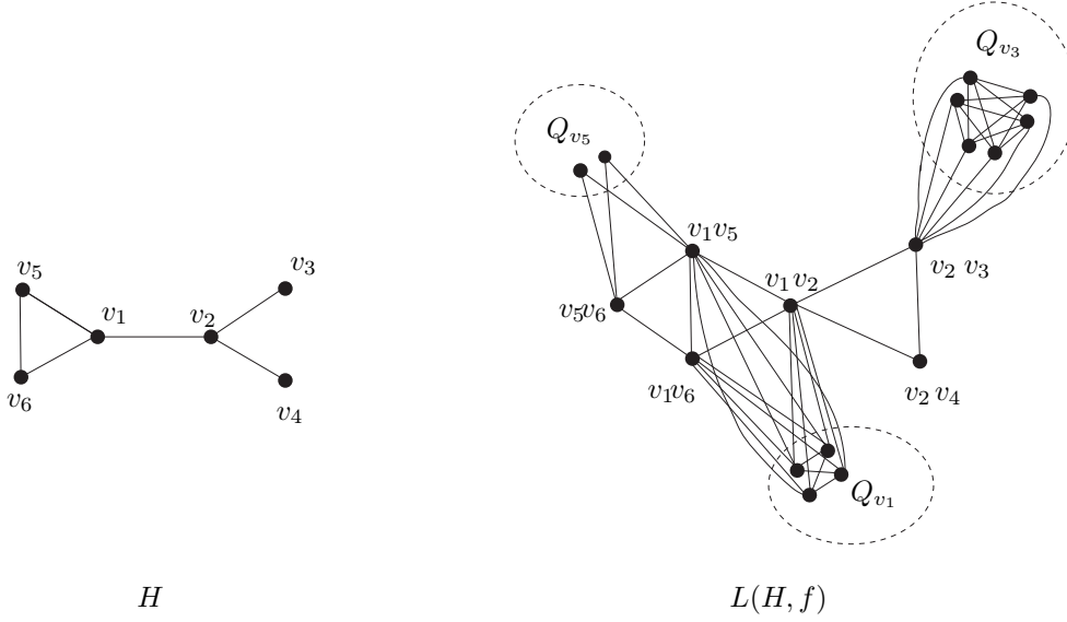
Fig. 1: A vertex-weighted graph (H, f) , where f : V(H) \rightarrow \mathbb{Z}_{\geq 0} is defined by f(v_1) = 2, f(v_3) = 3, f(v_5) = 1, f(v_2) = f(v_4) = f(v_6) = 0 , and its generalized line graph L(H, f)
