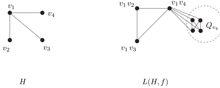
Fig. 4: A vertex-weighted graph (H, f) , where f : V(H) \rightarrow \mathbb{Z}_{\geq 0} is defined by f(v_1) = f(v_2) = f(v_3) = 0 and f(v_4) = 2 , and its generalized line graph L(H, f)
