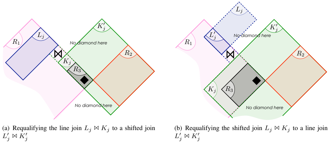
Fig. 19: The two cases where one needs to requalify the join in Claim 10.2.
