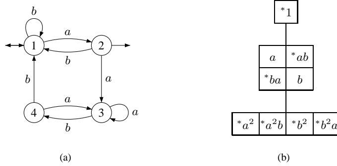
Fig. 1: Structural information about the language L
