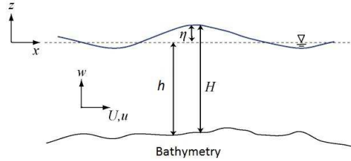
Figure 1: Depth averaged equations : notation
