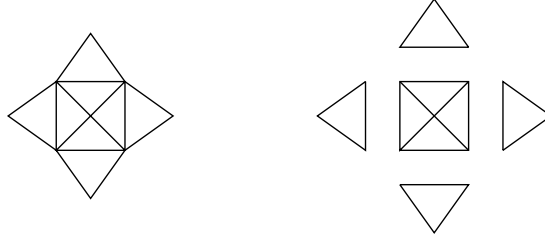
Figure 1: Clique-decomposition of a graph into five atoms.
